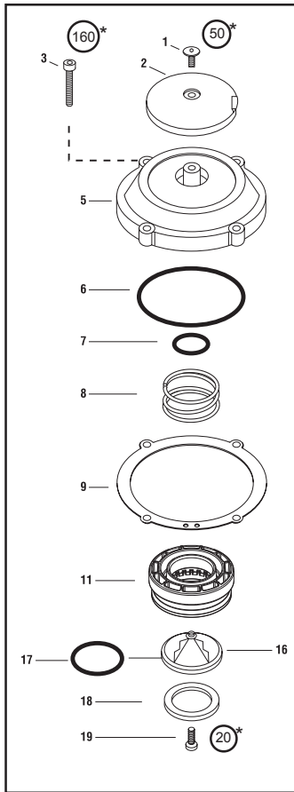
Cap and Valve Assembly 501056
