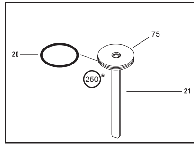
Piston Assembly 501519
